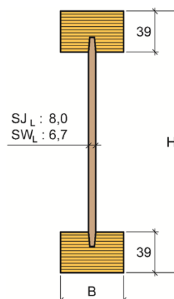
Fig. 1 Hunton I-bjelken m/ LVL flens.
